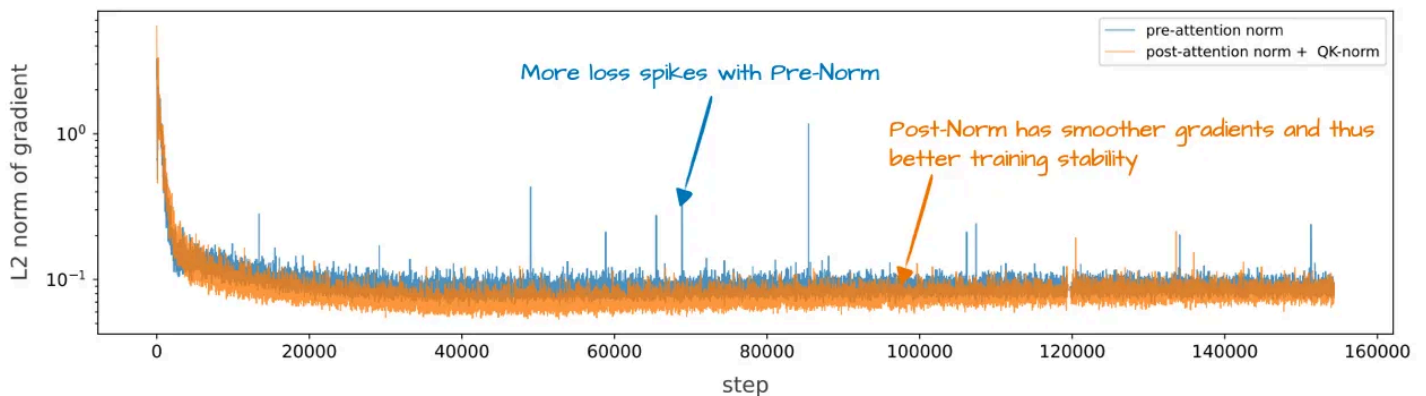
Figure 9: A plot showing the training stability for Pre-Norm (like in GPT-2, Llama 3, and many others) versus OLMo 2's flavor of Post-Norm. This is an annotated figure from the OLMo 2 paper, https://arxiv.org/abs/2501.00656
