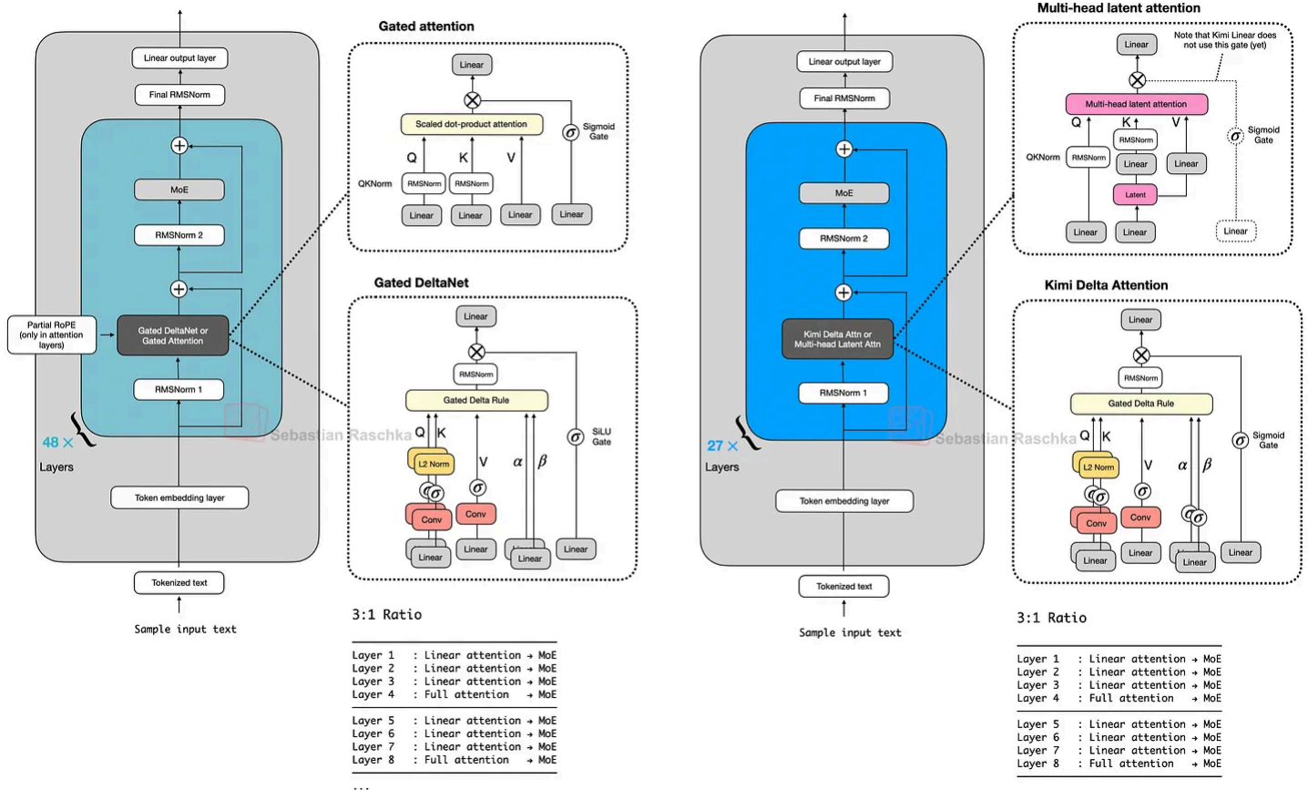
Figure 42: Qwen3-Next and Kimi Linear side by side.
