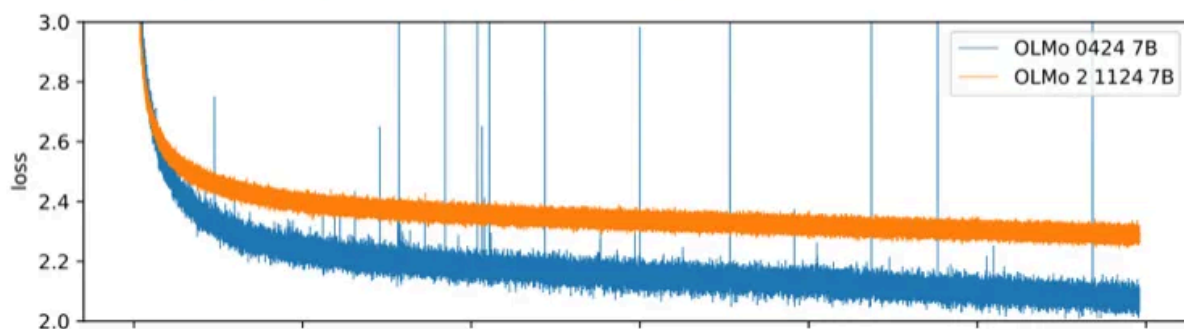
OLMo & OLMo 2 training loss curves
