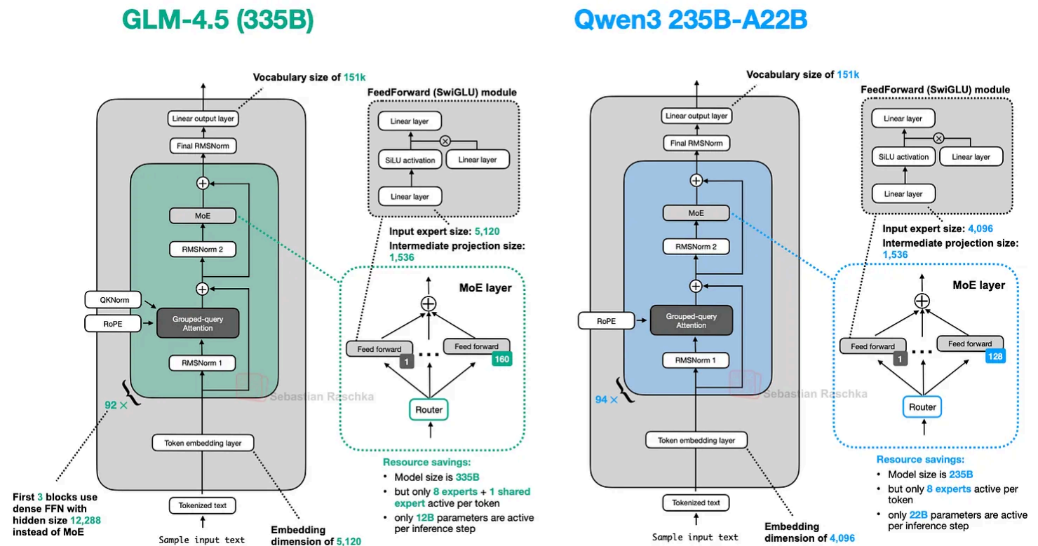
Figure 34: GLM-4.5 next to a similarly-sized Qwen3 model.
