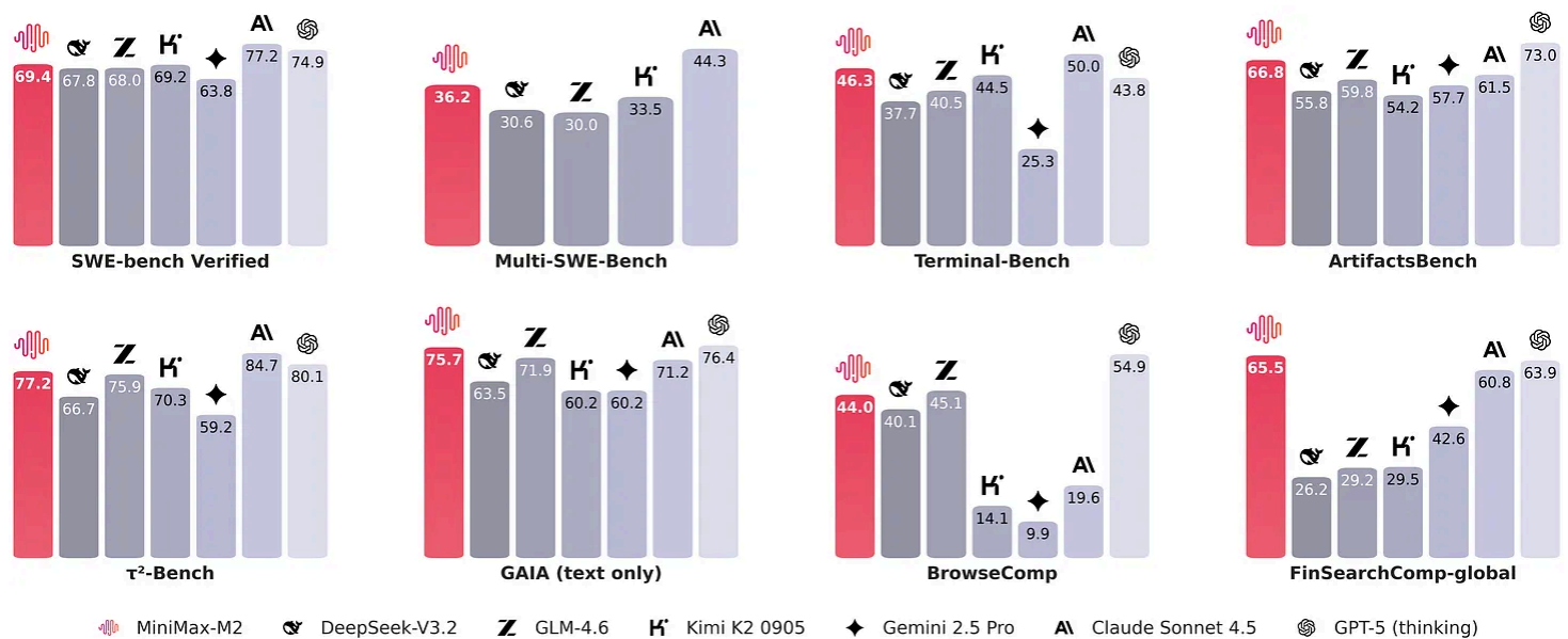
Figure 37: MiniMax-M2 benchmark performance compared to other popular open-weight and proprietary LLMs. Image from the official model hub release readme file.
