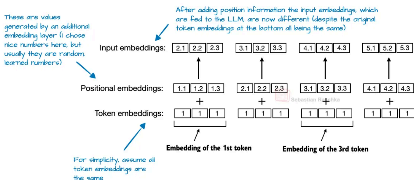
Figure 22: A modified figure from my Build A Large Language Model (From Scratch) book ( https://www.amazon.com/Build-Large-Language-Model-Scratch/dp/1633437167 ) illustrating absolute positional embeddings.
