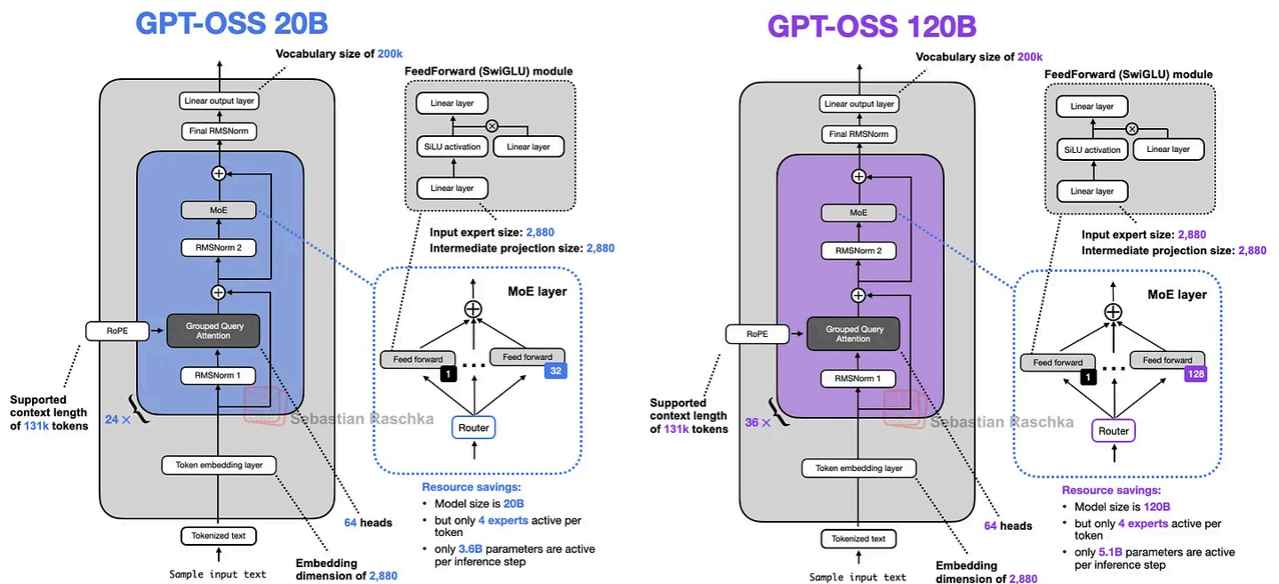
Figure 26: Architecture overview of the two gpt-oss models.
