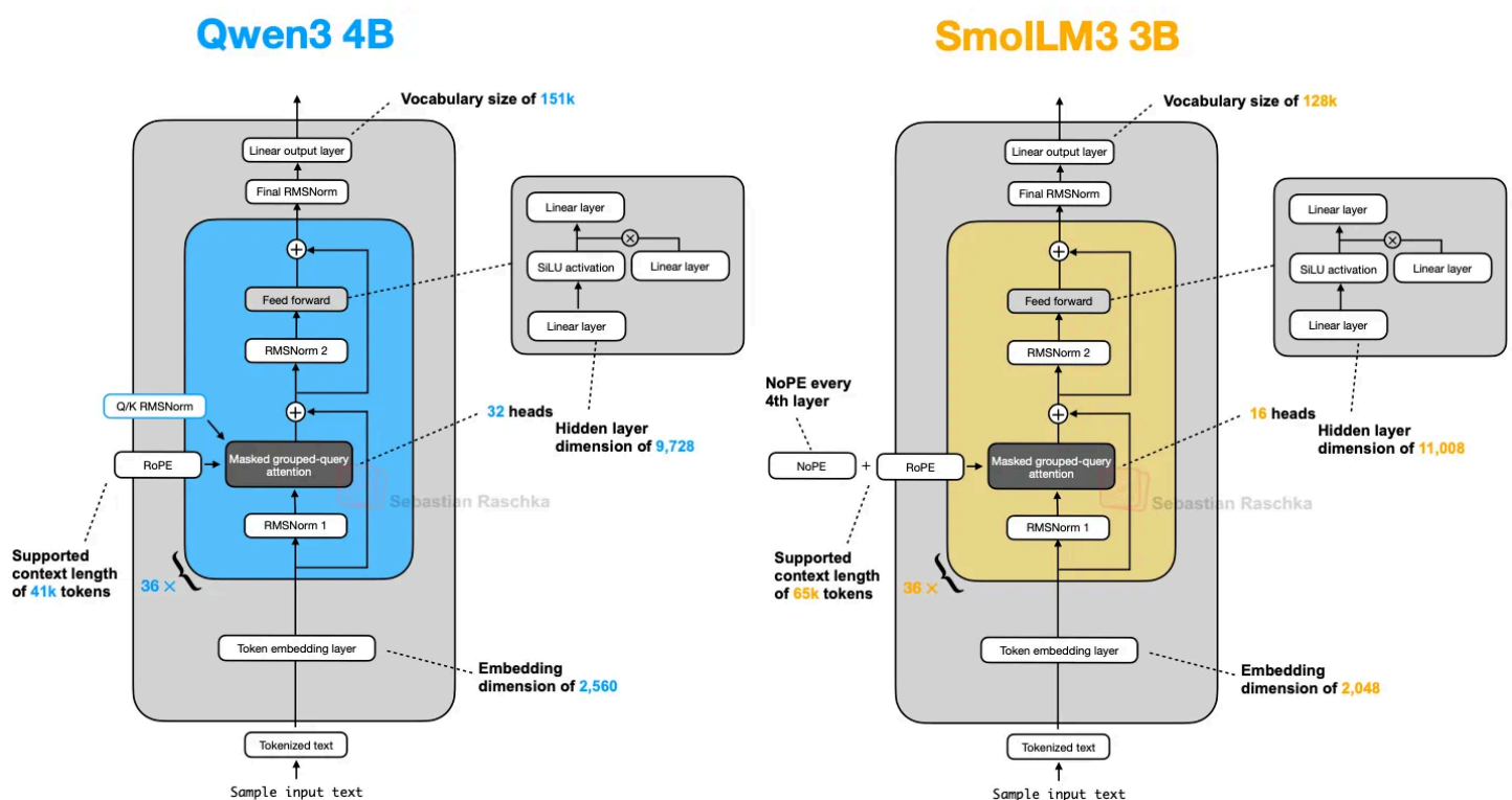
Figure 21: A side-by-side architecture comparison between Qwen3 4B and SmolLM3 3B.
