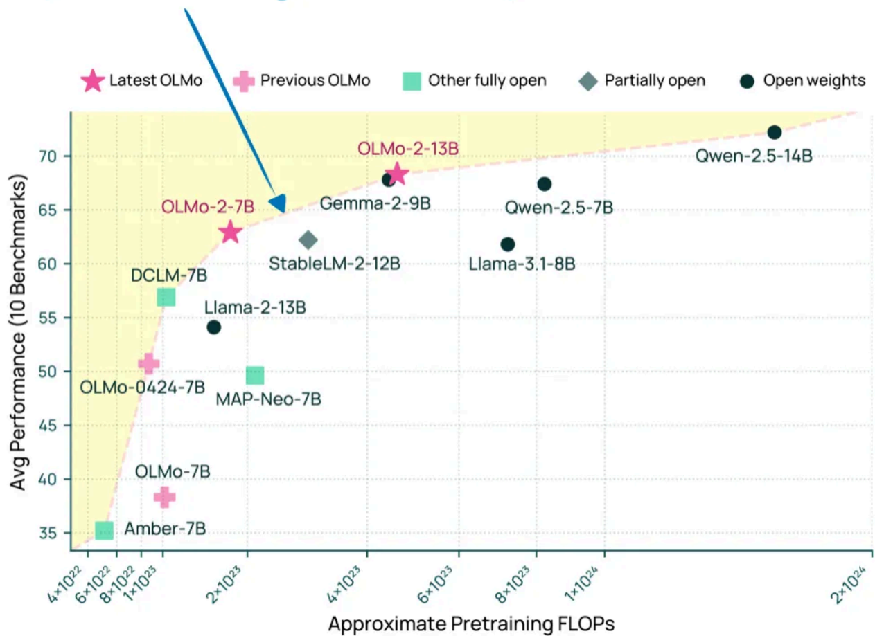
Figure 7: Modeling benchmark performance (higher is better) vs pre-training cost (FLOPs; lower is better) for different LLMs. This is an annotated figure from the OLMo 2 paper, https://arxiv.org/abs/2501.00656
