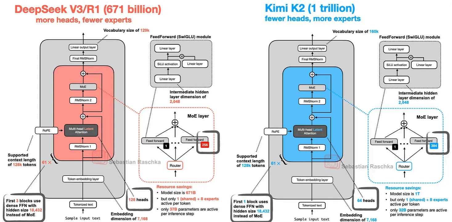
Figure 25.1: An architecture comparison between DeepSeek V3 and Kimi K2.
