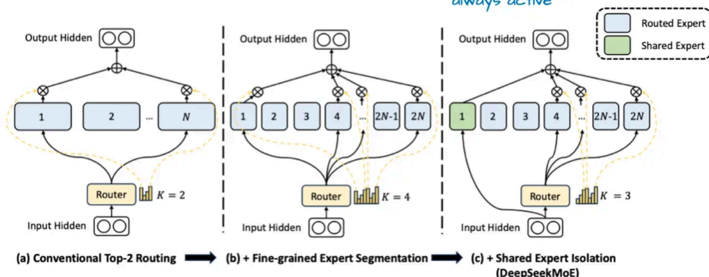
Figure 6: An annotated figure from "DeepSeekMoE: Towards Ultimate Expert Specialization in Mixture-of-Experts Language Models", https://arxiv.org/abs/2401.06066
