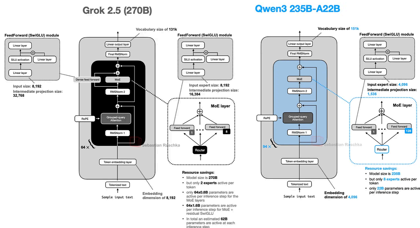
Figure 32: Grok 2.5 next to a Qwen3 model of comparable size
