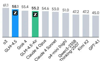
Figure 33: GLM-4.5 benchmark from the official GitHub repository at https://github.com/zai-org/GLM-4.5
