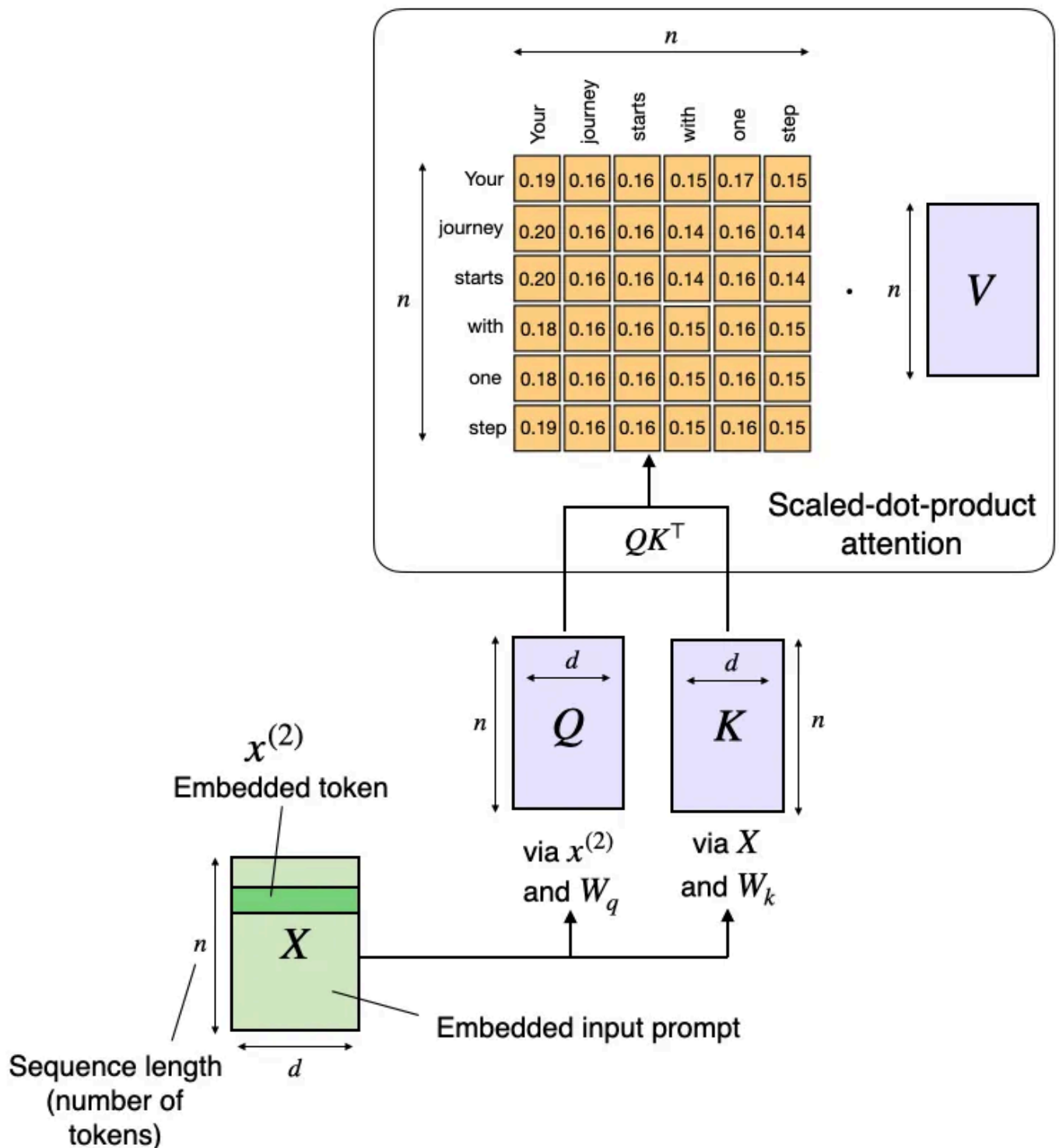
Figure 40: Illustration of the quadratic cost in attention due to sequence length n .
