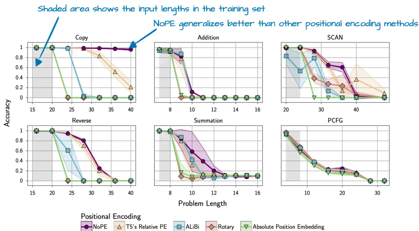
Figure 23: An annotated figure from the NoPE paper ( https://arxiv.org/abs/2305.19466 ) showing better length generalization with NoPE.
