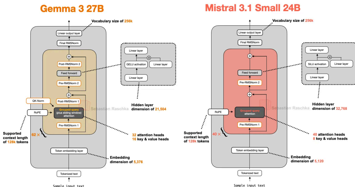
Figure 16: An architecture comparison between Gemma 3 27B and Mistral 3.1 Small 24B.
