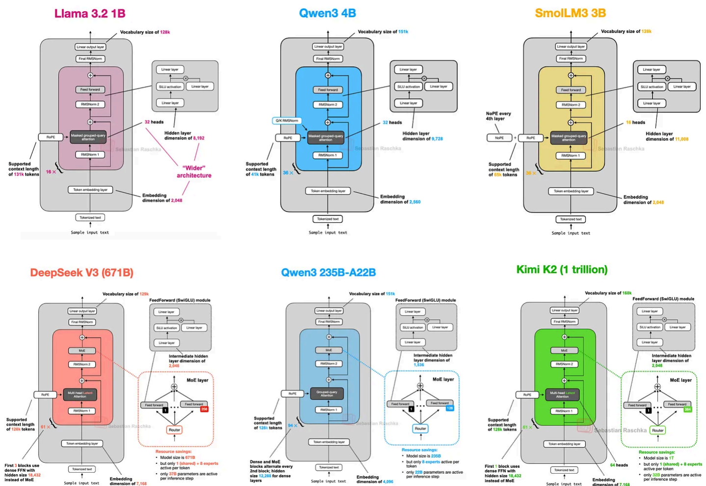
Figure 1: A subset of the architectures covered in this article.
