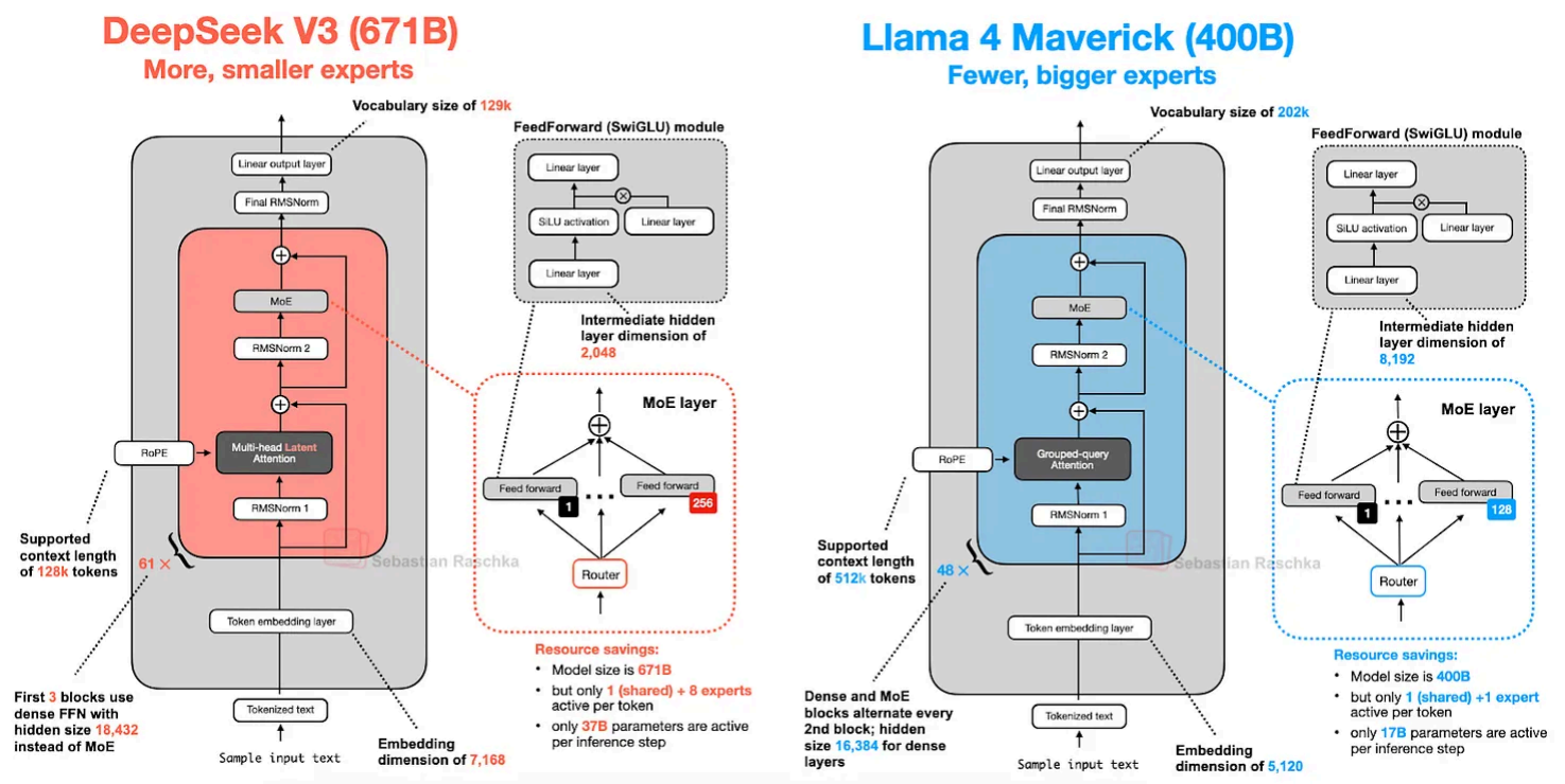
Figure 17: An architecture comparison between DeepSeek V3 (671-billion parameters) and Llama 4 Maverick (400-billion parameters).
