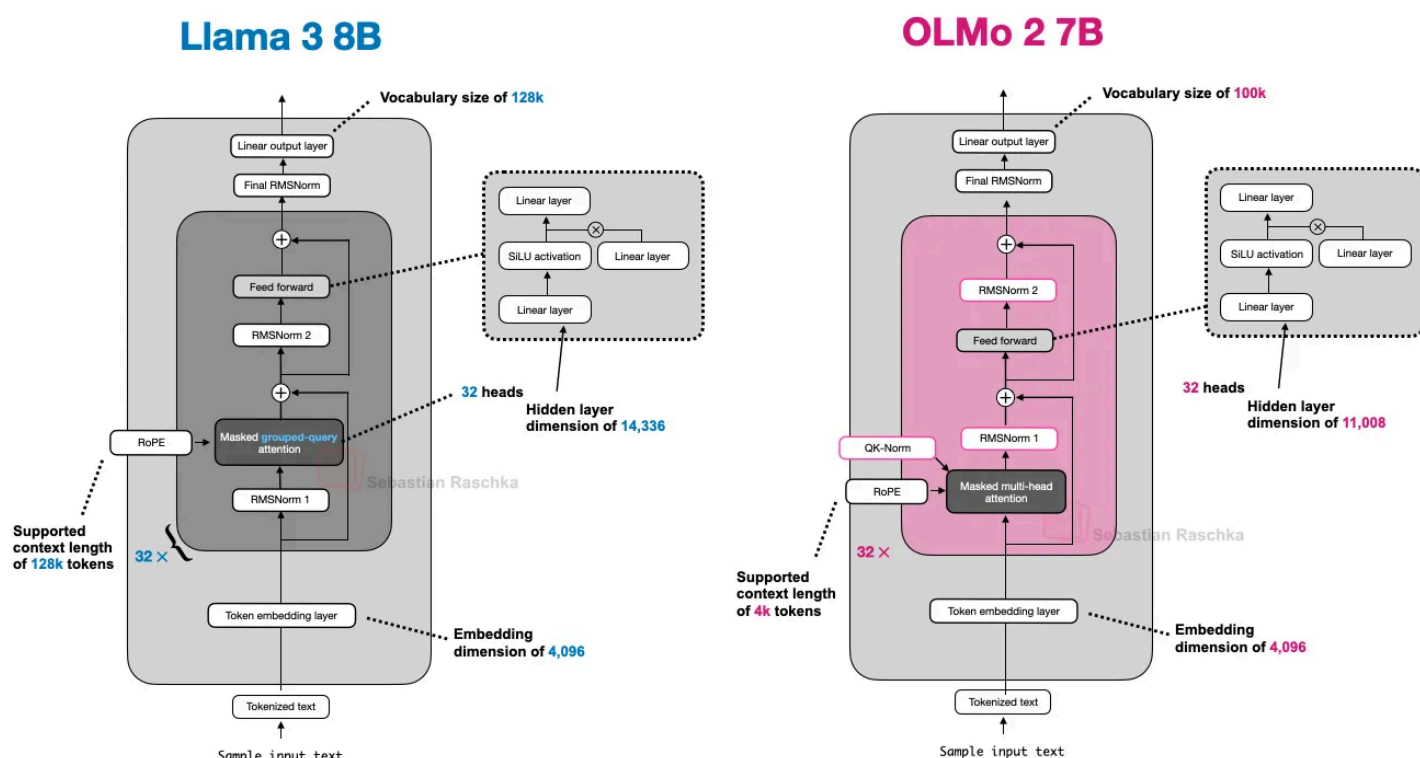
Figure 10: An architecture comparison between Llama 3 and OLMo 2.
