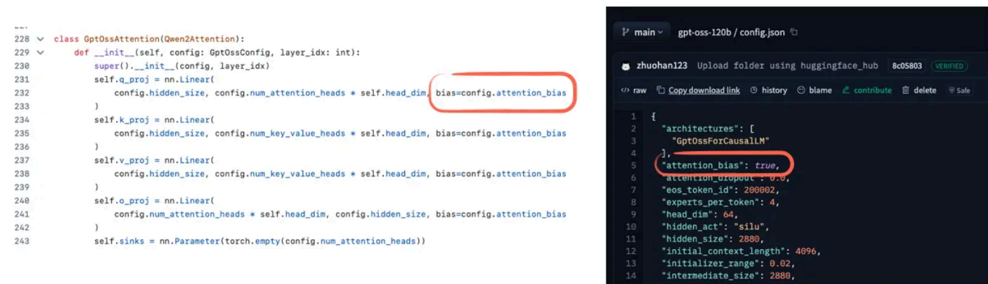
Figure 29: gpt-oss models use bias units in the attention layers. See code example here.
