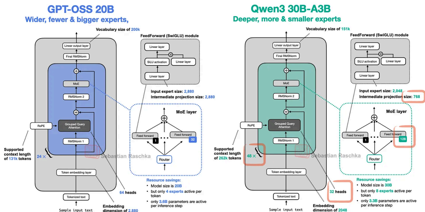
Figure 27: Architecture comparison between gpt-oss and Qwen3
