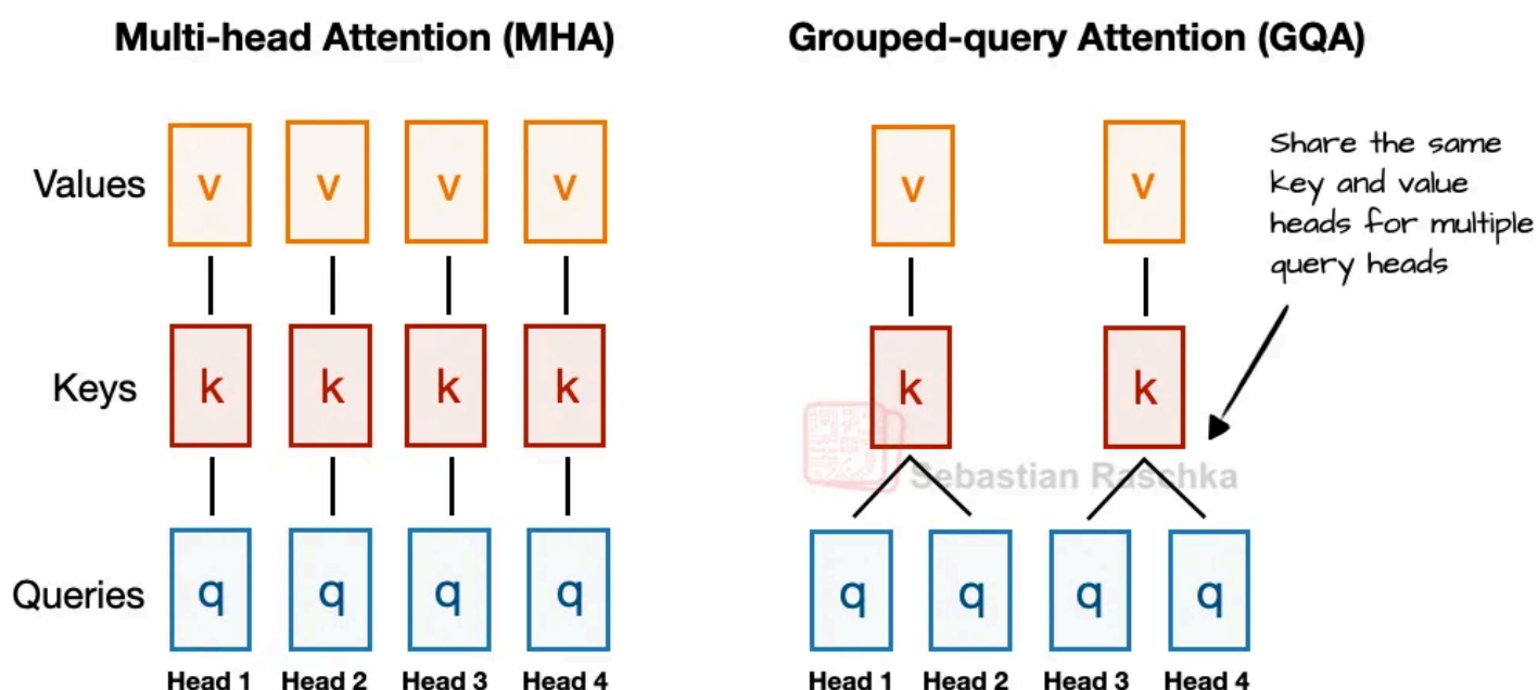
Figure 2: A comparison between MHA and GQA. Here, the group size is 2, where a key and value pair is shared among 2 queries.
